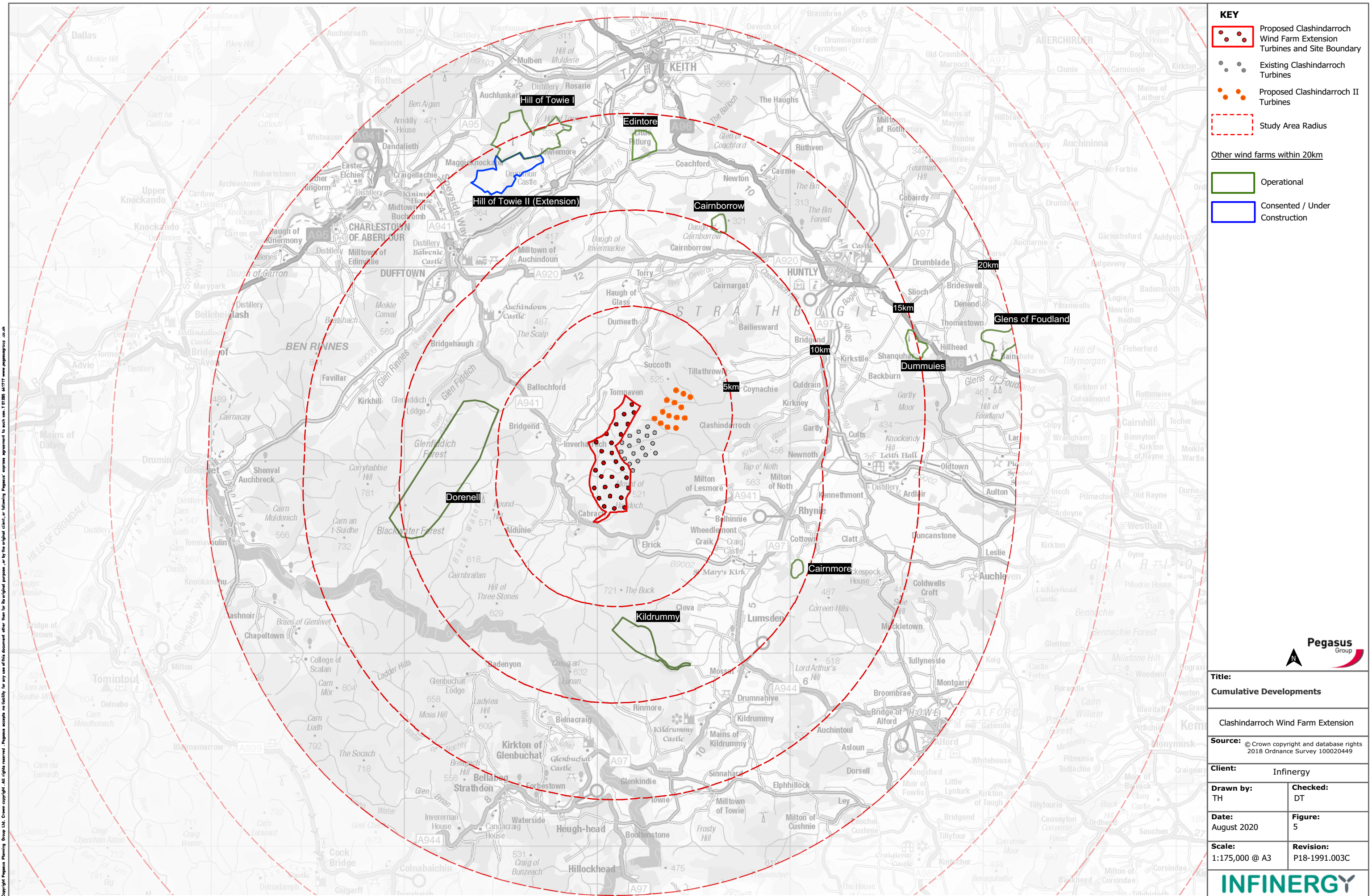
Figure 5: Cumulative Developments
